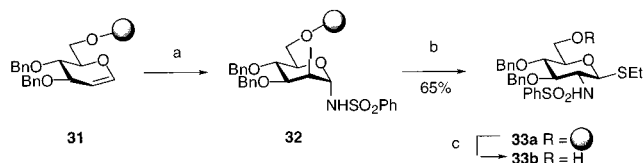
Scheme 10. Synthesis of a Polymer-Bound Thioethyl 2-Amido-Glycosyl Donor a
